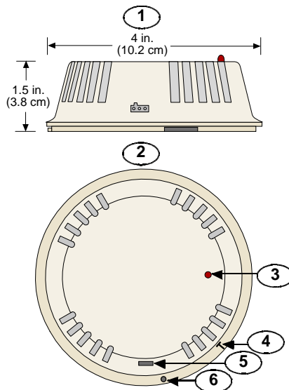
Figure 1: D7050/D7050TH Side and Top Views
